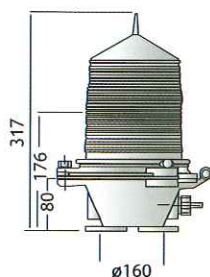
Type RL-133LS
